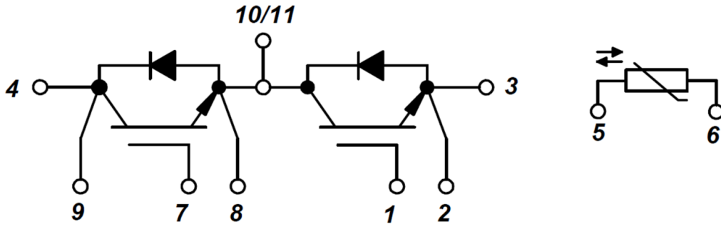
Figure 14. Circuit Diagram
