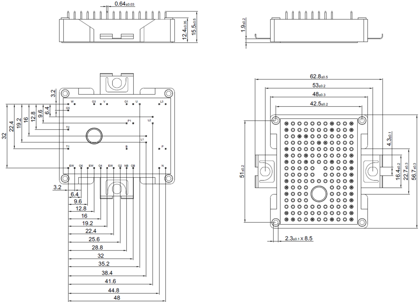
Dimensions in (mm) Figure 18. Package Outline
