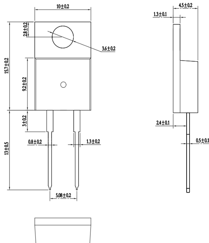
Figure 8. Package Outline
