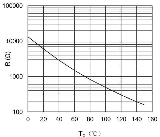
Figure 14. NTC Characteristics
