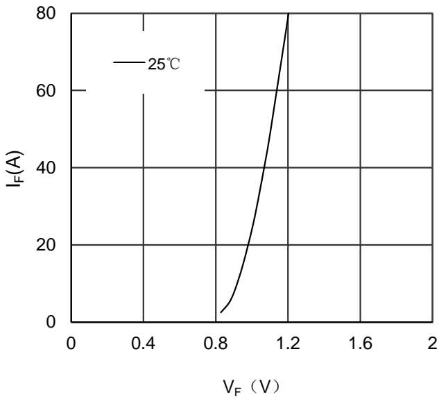
Figure 11. Diode Forward Characteristics Diode-rectifier
