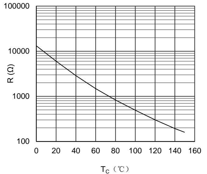
Figure 14. NTC Characteristics
