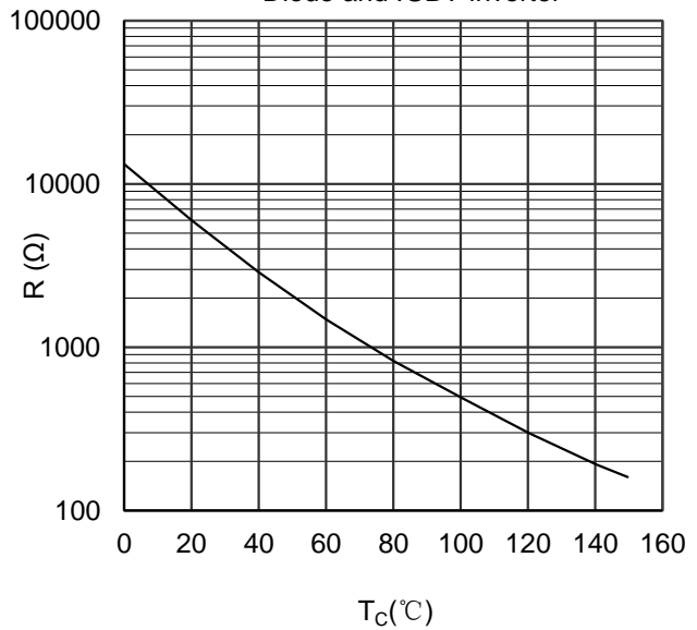
Figure 13. NTC Characteristics
