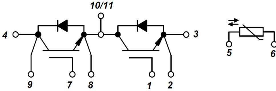
Figure 14. Circuit Diagram
