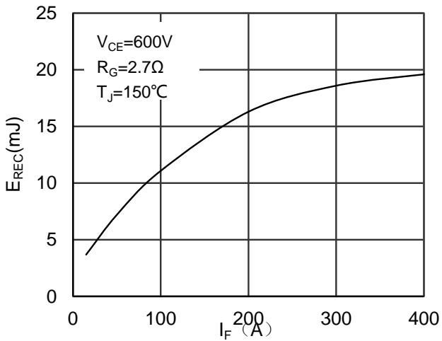
Figure 11. Switching Energy vs Forward Current Diode-
