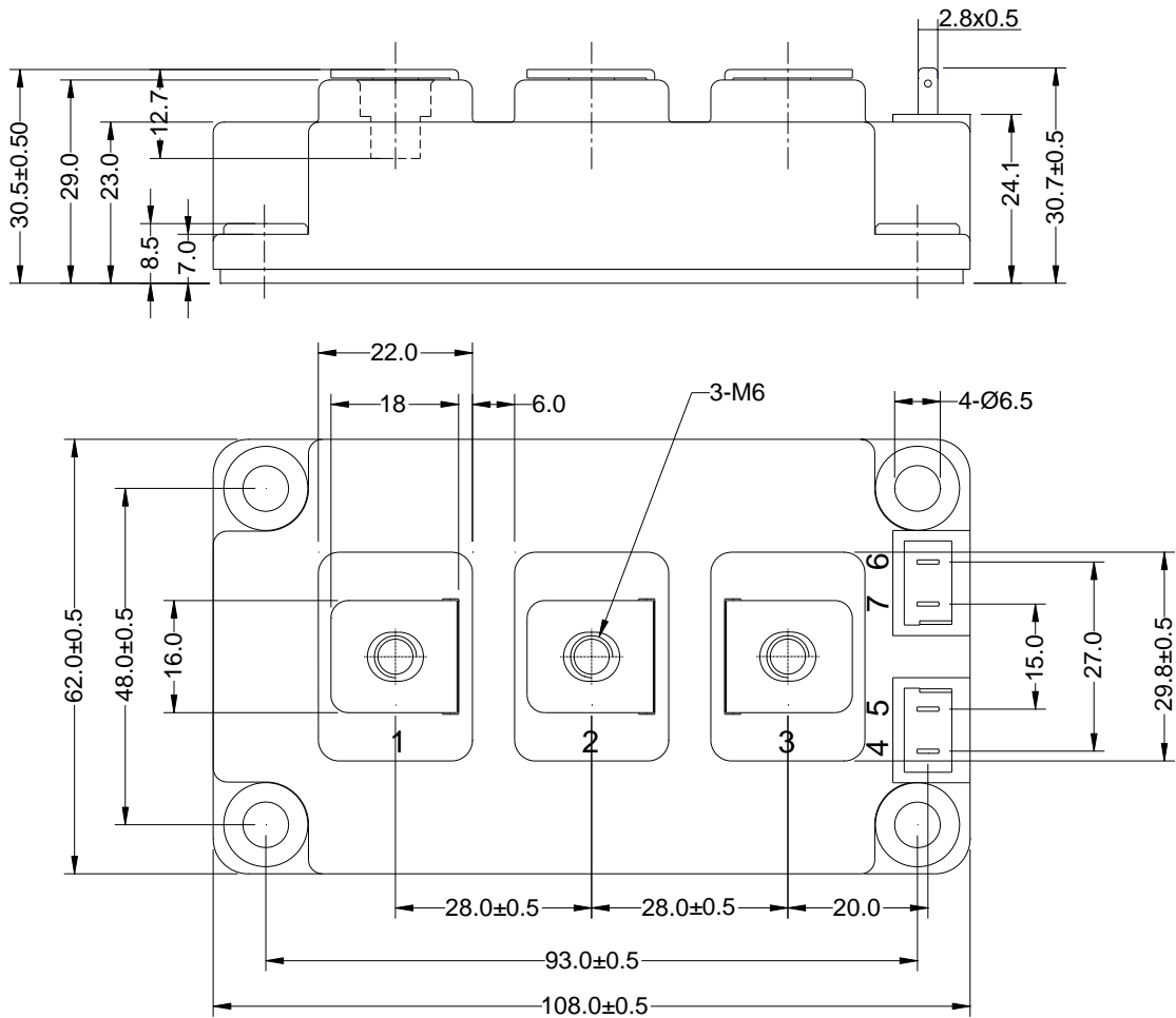
Dimensions in (mm) Figure 14. Package Outline
