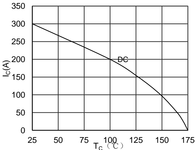
Figure 7. Collector Current vs Case temperature IGBT-inverter
