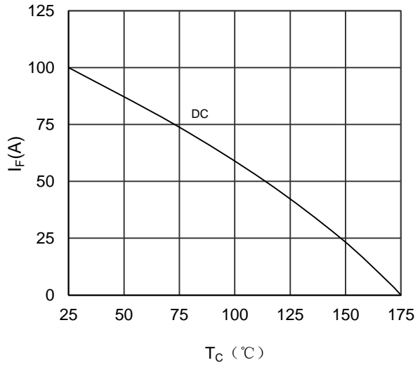
Figure 12. Forward current vs Case temperature Diode-inverter
