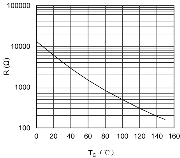
Figure 13. NTC Characteristics
