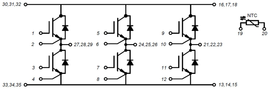
Figure 14. Circuit Diagram
