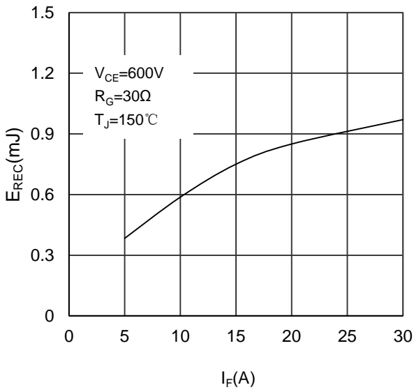
Figure 9. Switching Energy vs Forward Current Diode-inverter
